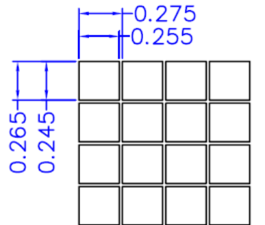
DETAIL FOR DOTS 16:1
