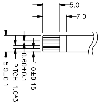
DETAIL A SCALE 2.0
