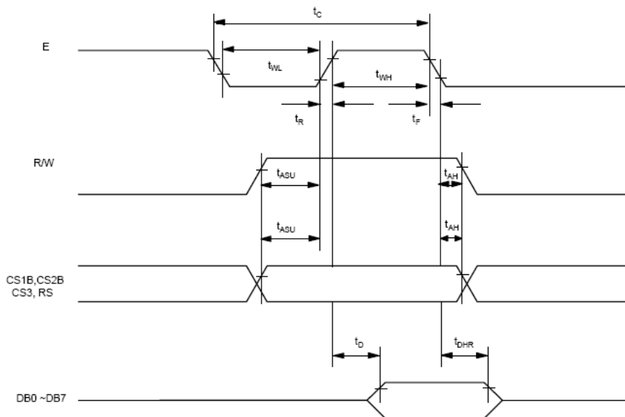
Figure 2. Read Timing
